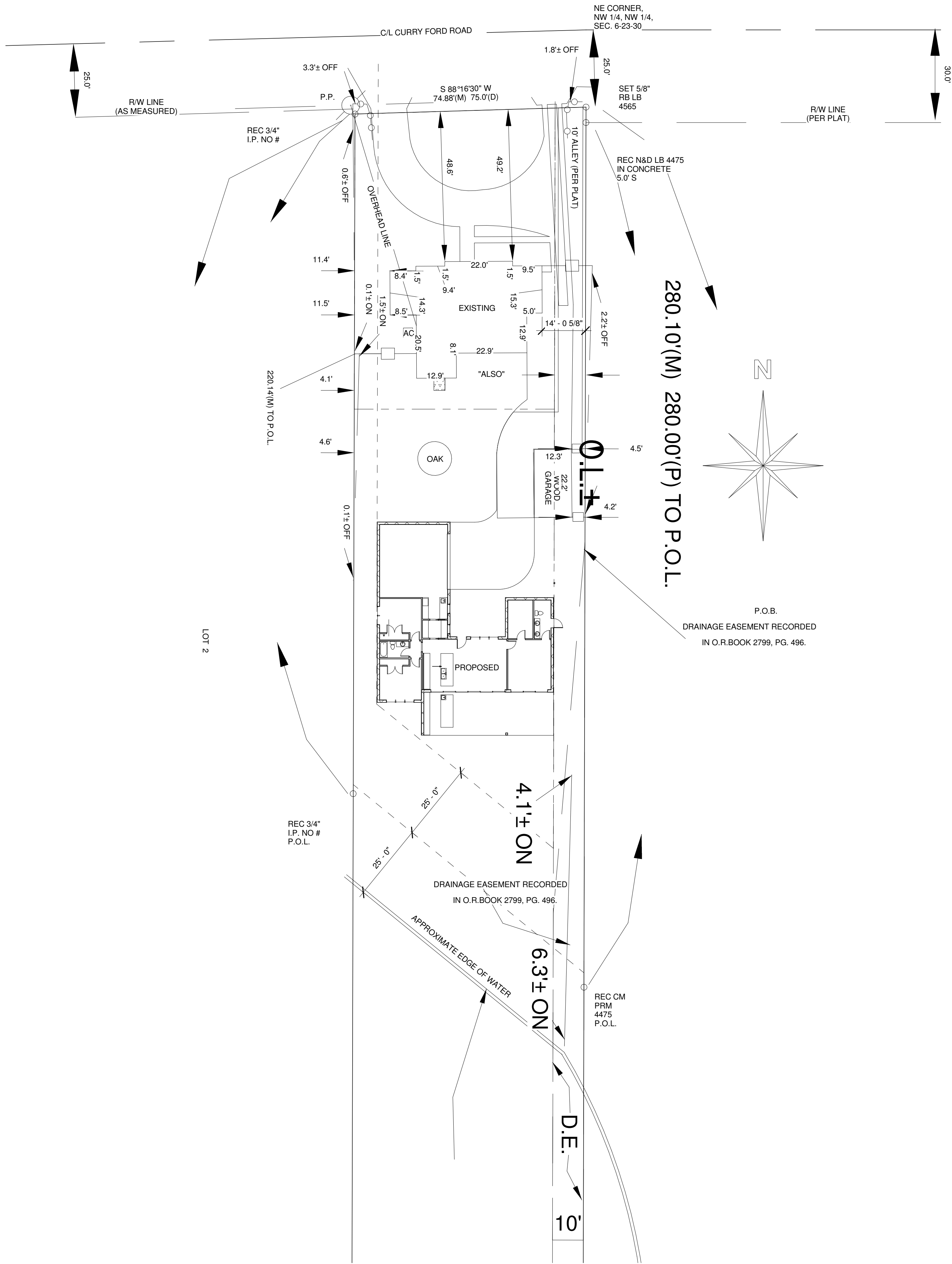
1 SITE PLAN 1" = 20'-0"
