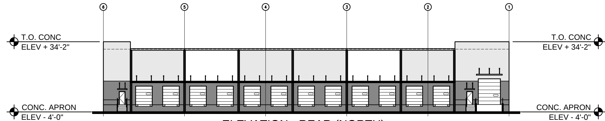
ELEVATION - REAR (NORTH)
