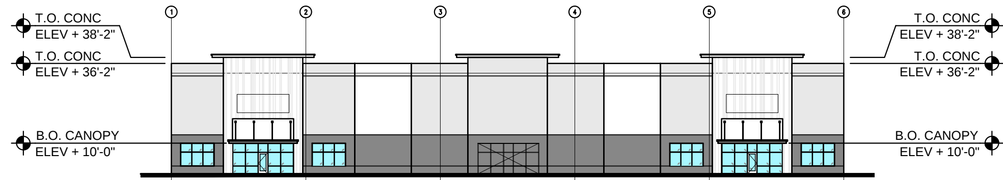
ELEVATION - FRONT (SOUTH)
