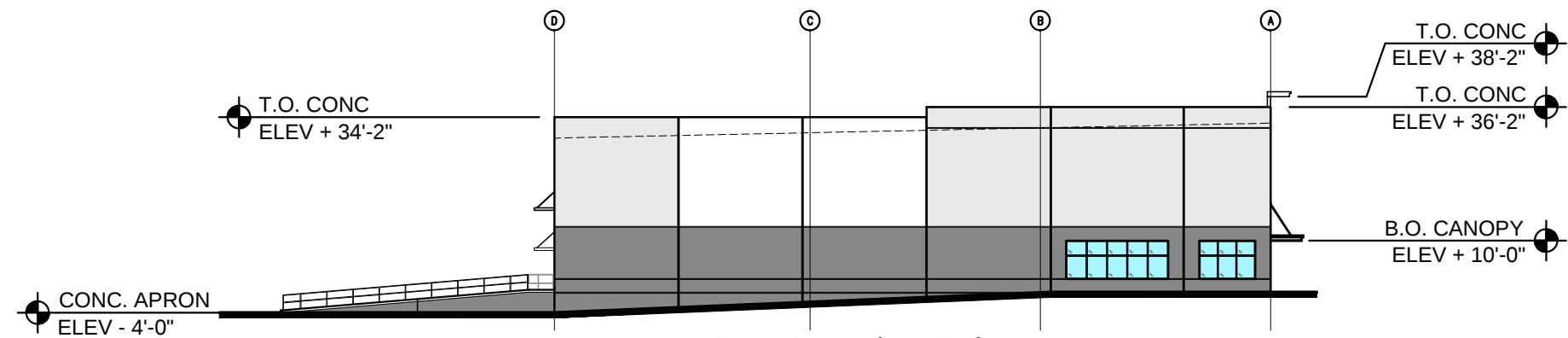
ELEVATION - SIDE (WEST)
