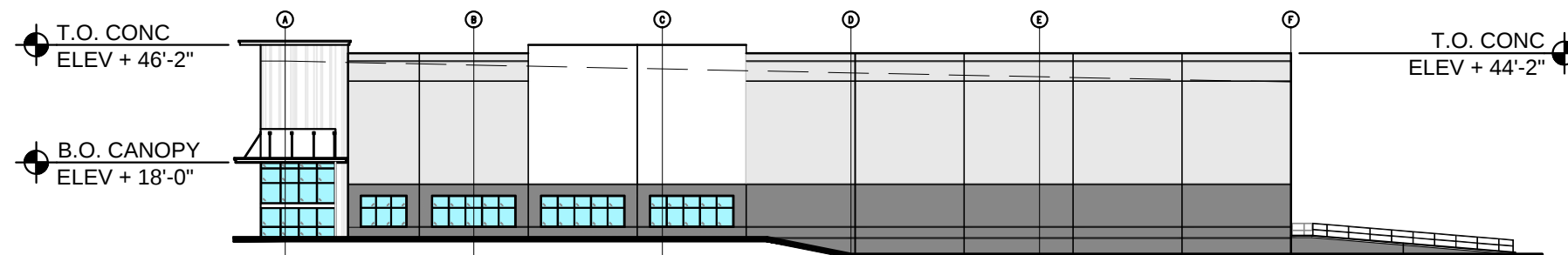
ENLARGED ELEVATION - SIDE
