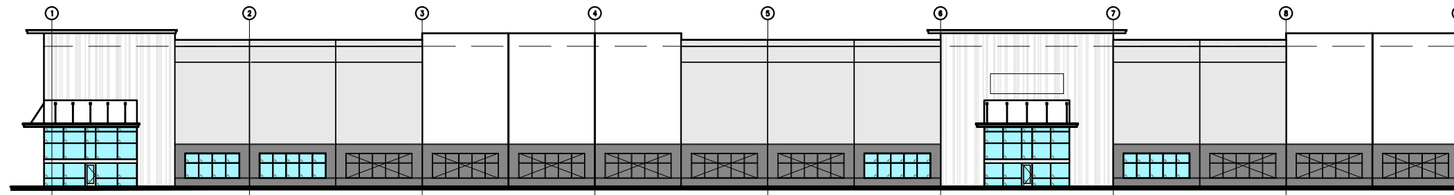
ENLARGED ELEVATION - FRONT
